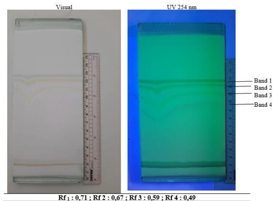
Figure 2. Band from preparative thin layer chromatography
