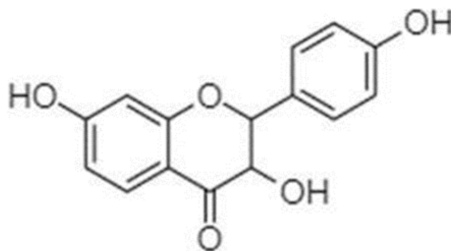
Figure 2. Interpretation of 3, 7, 4' trihydroxy flavone spectra
